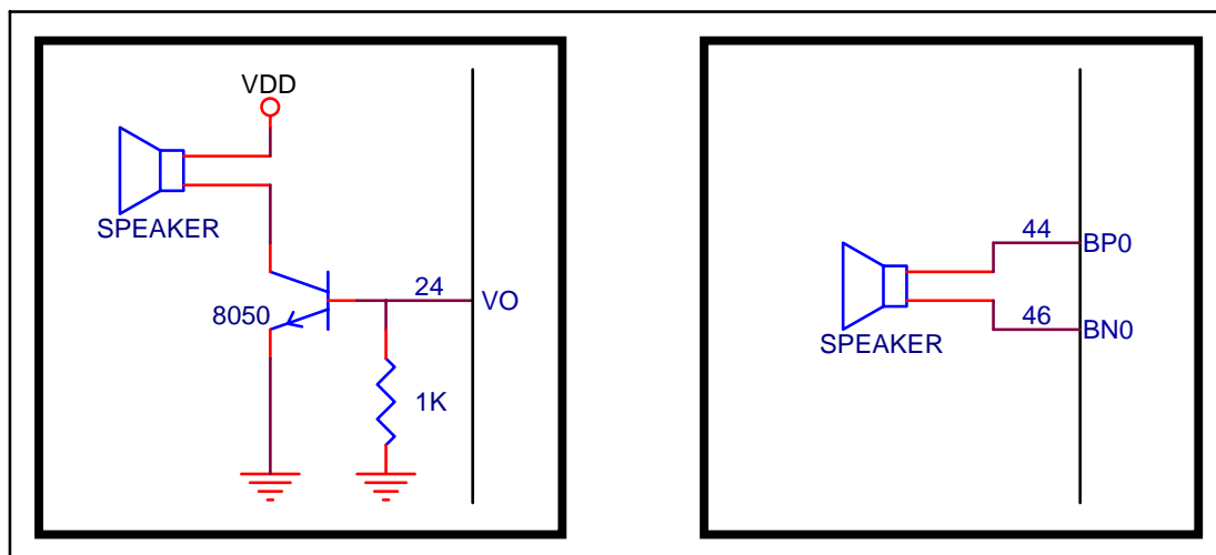
DAC output
