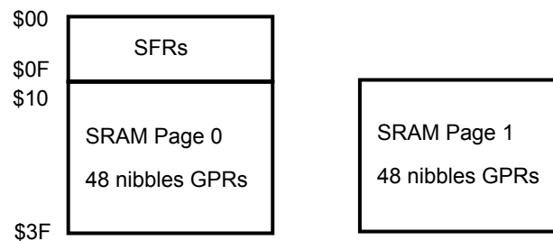
FIGURE 2: SRAM Map of AM4HAxxxx
