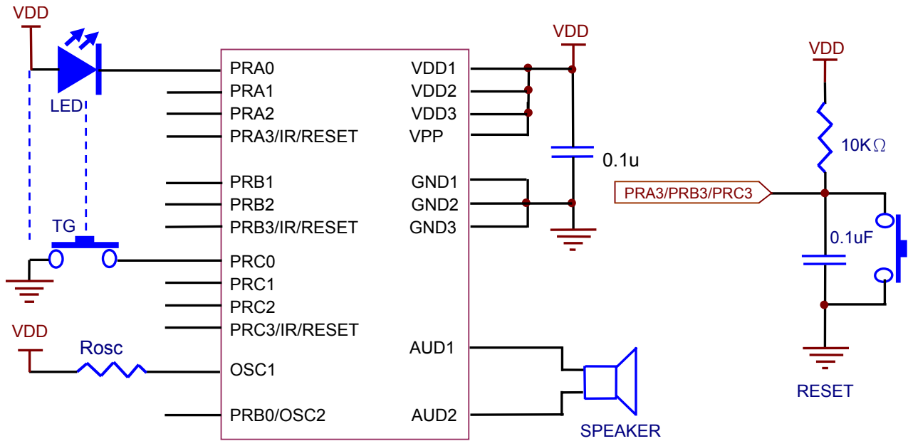
AM4HA250A Push-Pull Driving *
