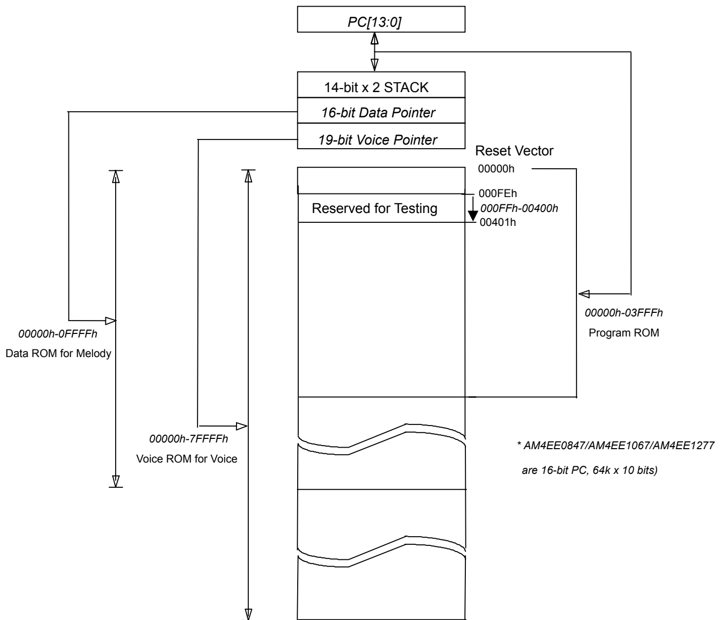
FIGURE 1 : ROM Map of AM4EE Series
